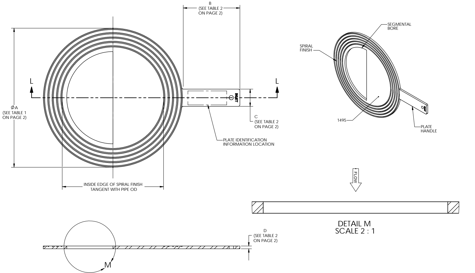
SECTION L-L
