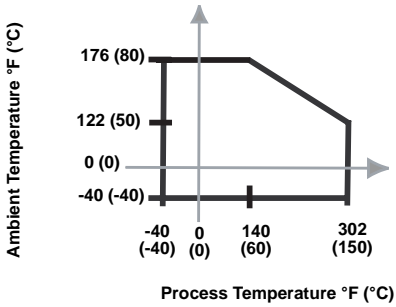
Figure A-2. Temperature
