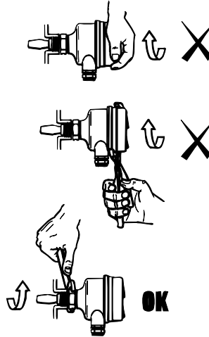
Figure 2-2. Tighten the Switch
