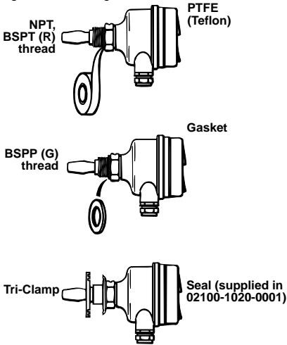
Figure 2-1. Sealing
