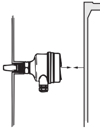
Figure 1-3. Ensure Adequate Space Outside Tank
