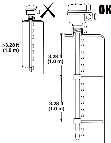
Figure 1-5. Support fork if high dynamic loads.
