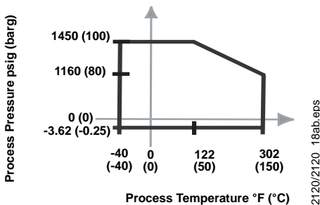
Figure A-1. Process Pressure
