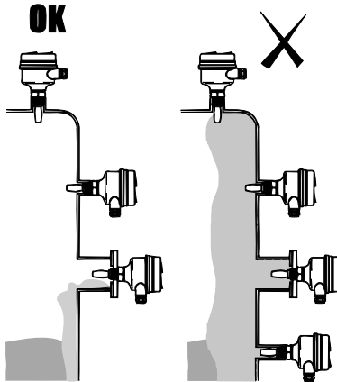
Figure 1-4. Example of ok and not ok build-up on tank wall.
