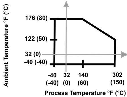
FIGURE 3. Temperature
