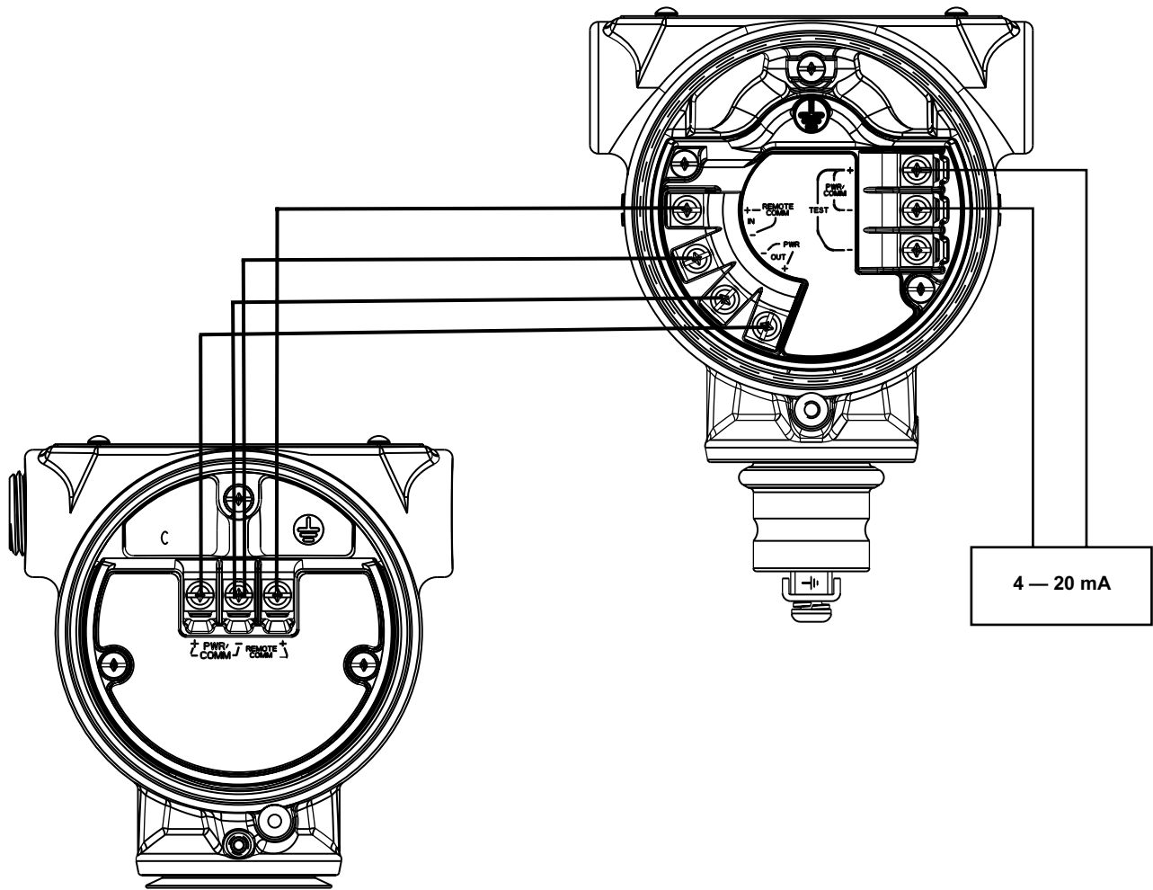
Figure 1-1. Remote Mount Meter wiring diagram
